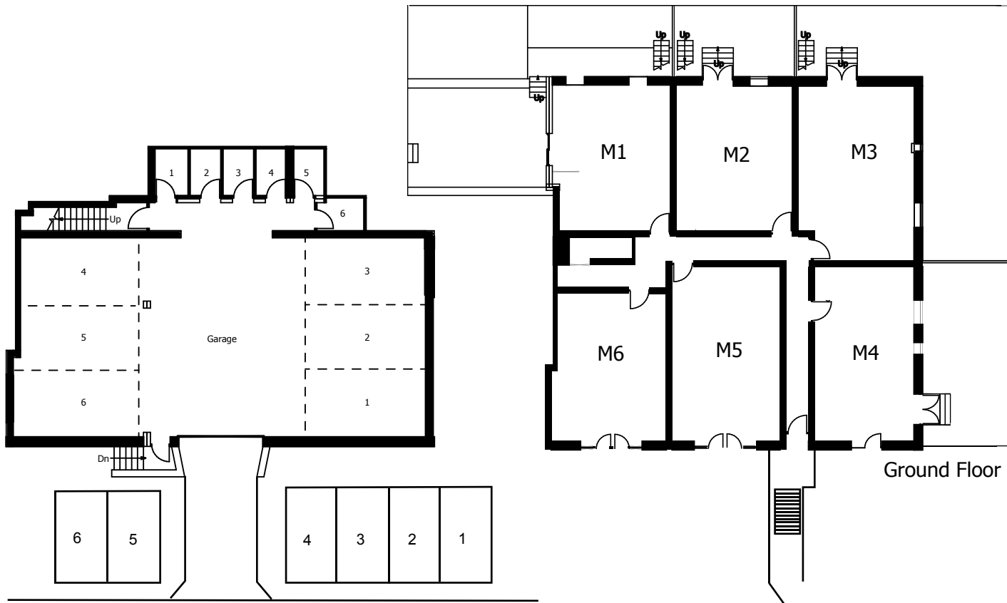
Lower Ground Floor Parking and Stores
