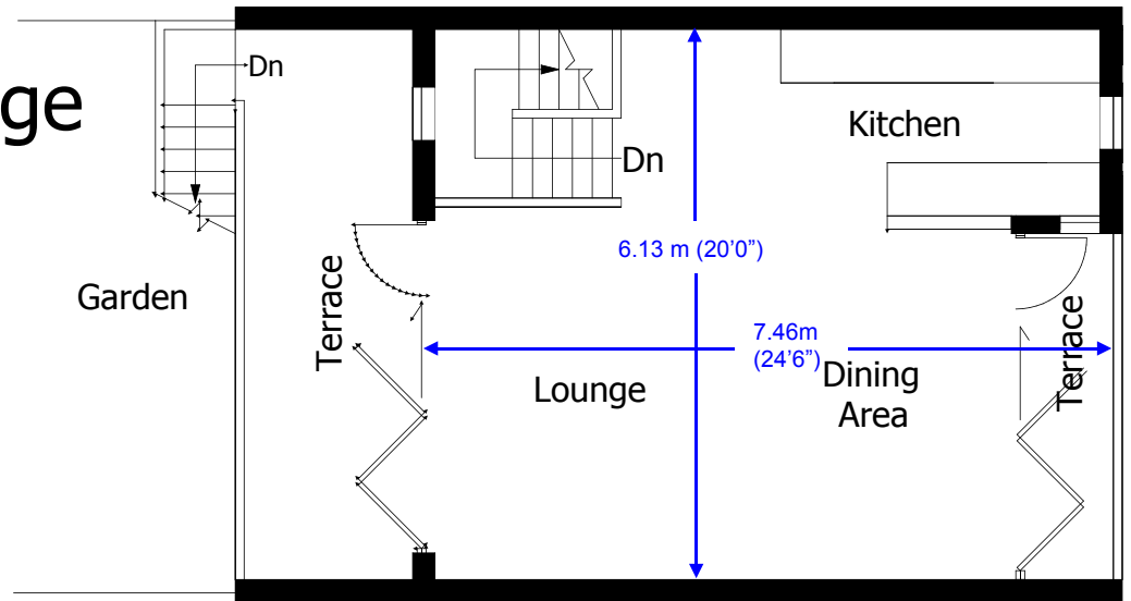
Second Floor
